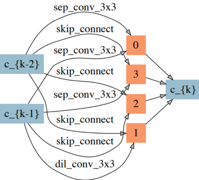
Normal cell
