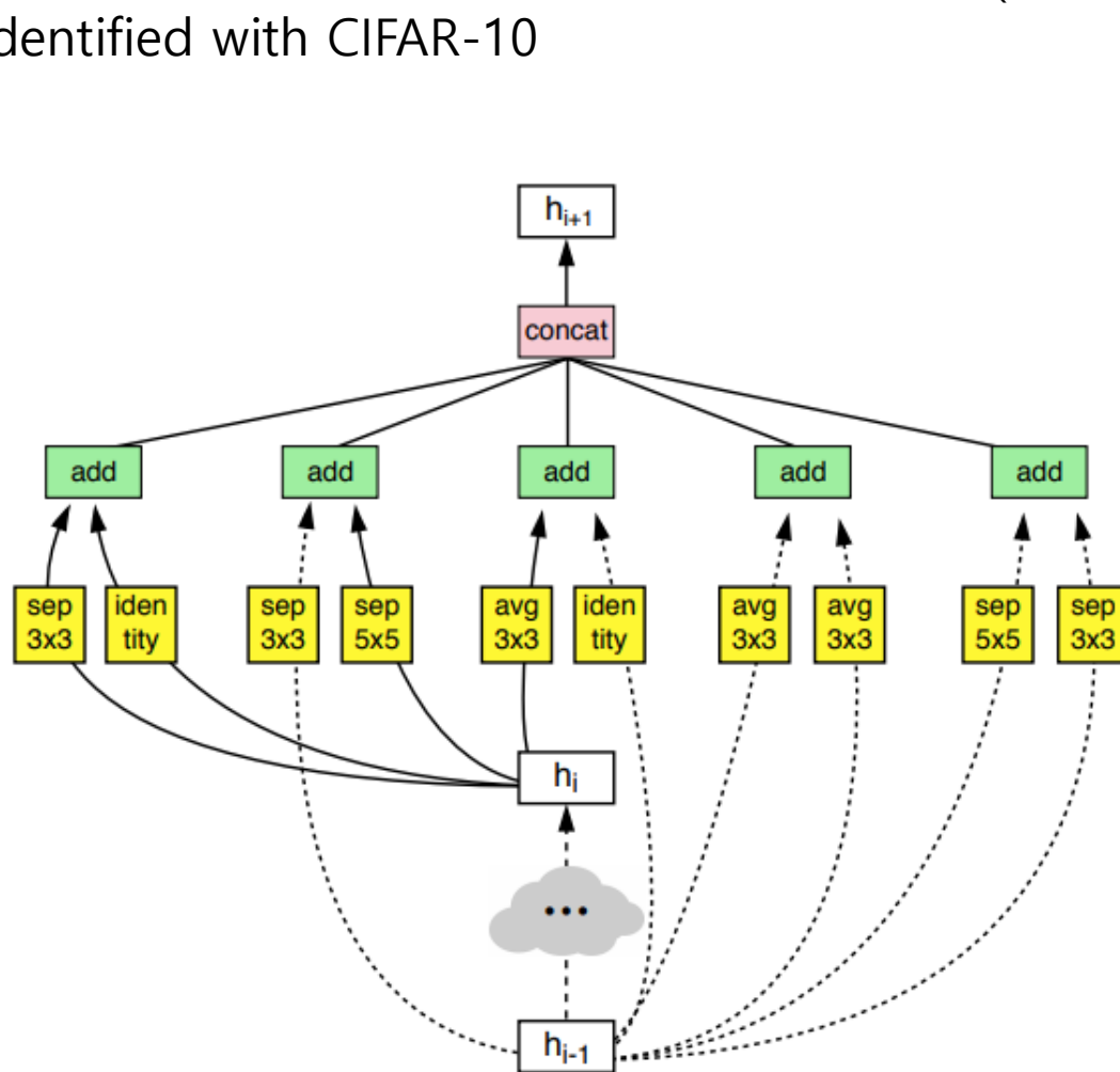
Normal Cell
