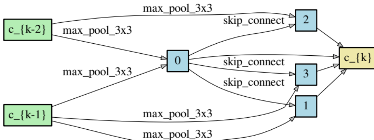
Reduction cell learned on CIFAR-10.
