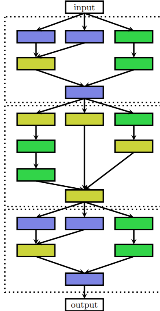
an architecture built by stacking the cells sequentially
