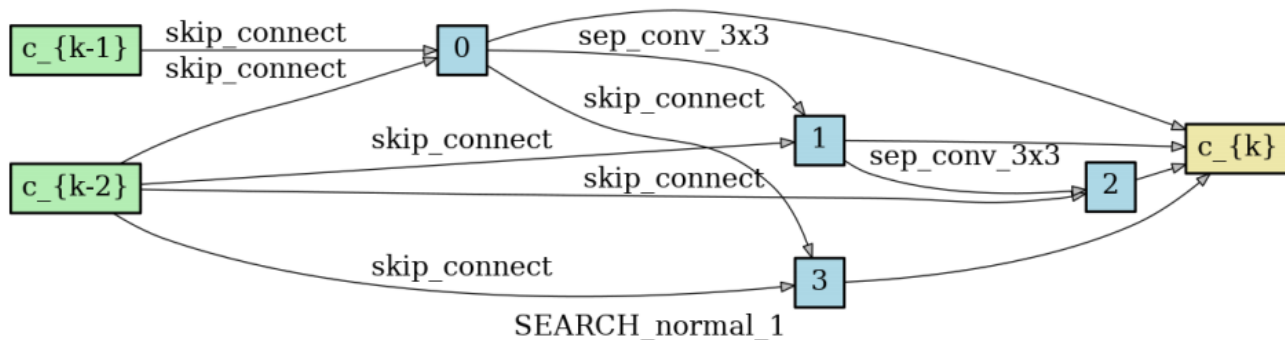
(b) Middle Cells
