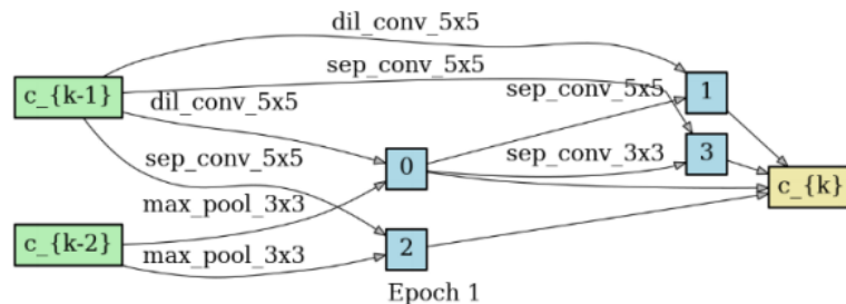
(b.2) Searching with early stopping
