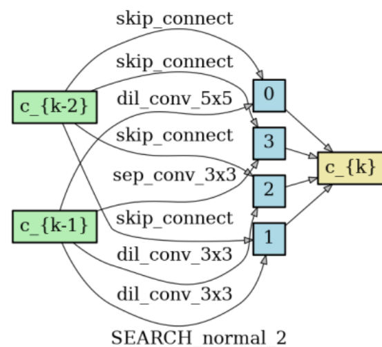
(c) Last Cells
