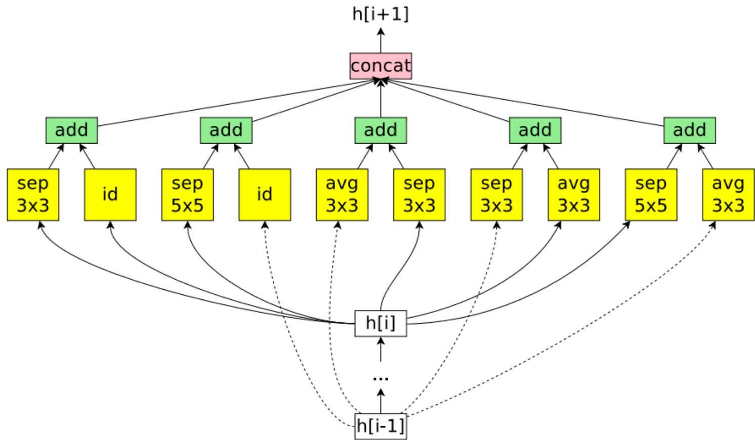
Convolution cell
