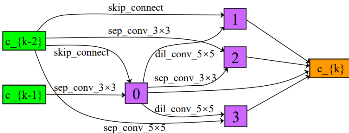
(a) Stage 1, CIFAR10 Test Err. 2.90%
