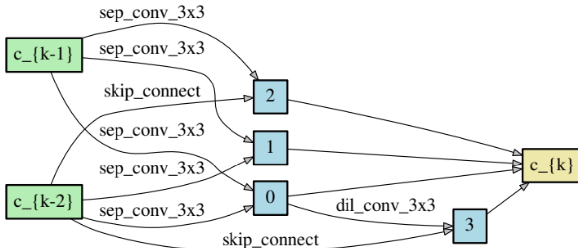
Normal cell learned on CIFAR-10
