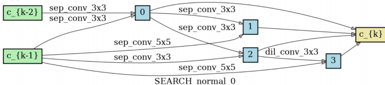
(b) Middle Cells
