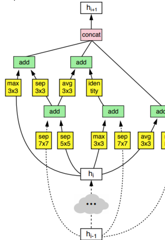
Reduction Cell
