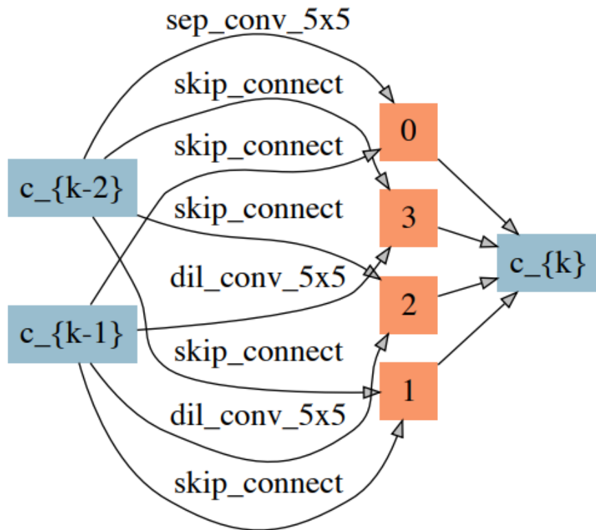
Normal cell
