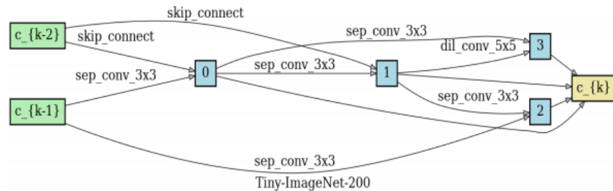
Reduction cell
