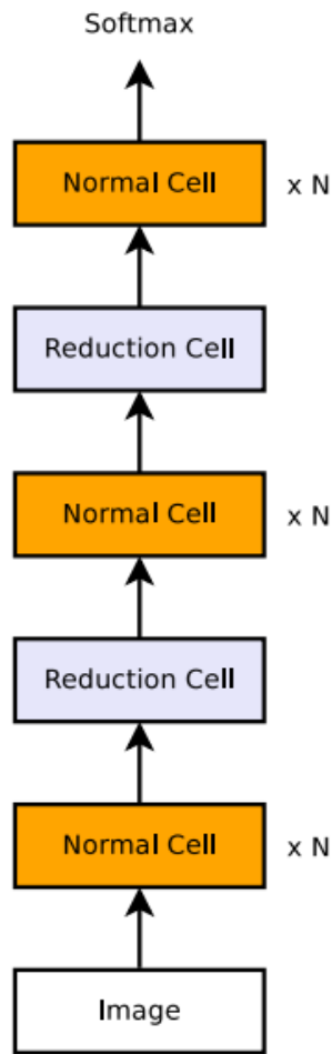
CIFAR10 Architecture
