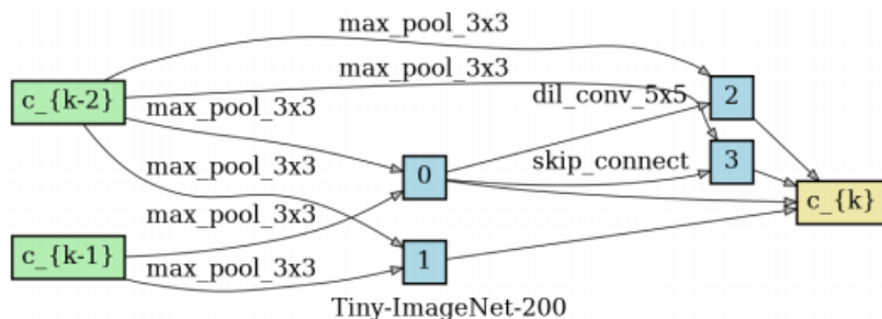
Reduction cell
