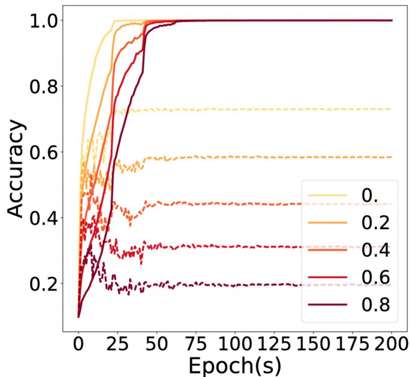
(b) Noise added on classification labels.
