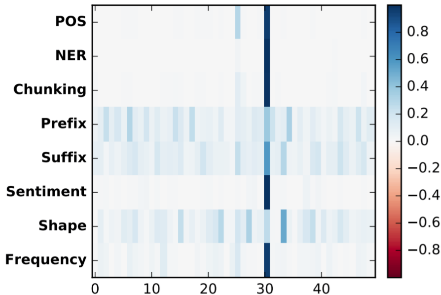
(c) GloVe, no dropout.
