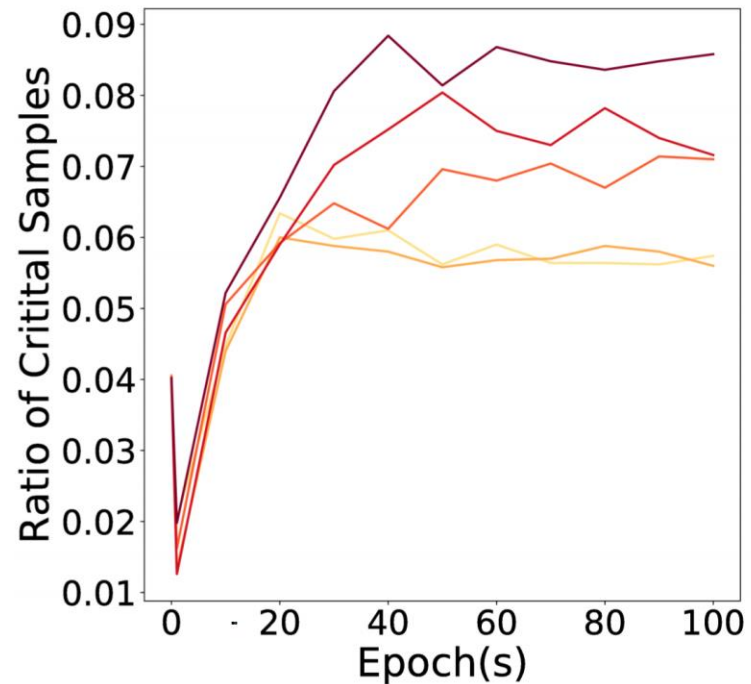
(a) Noise added on classification inputs.
