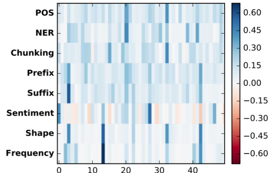
(b) Word2vec, with dropout.
