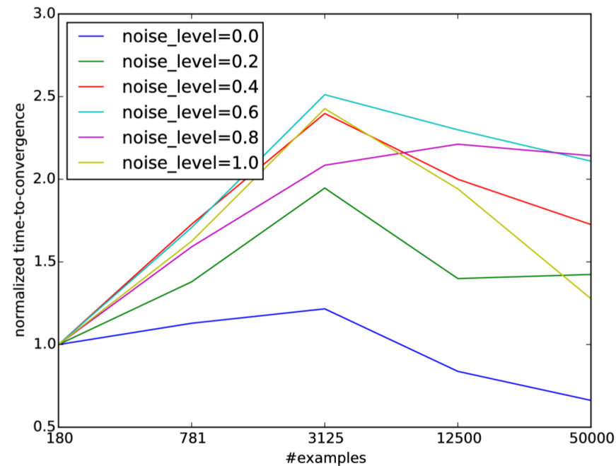
Dataset size with capacity fixed to 4096 units
