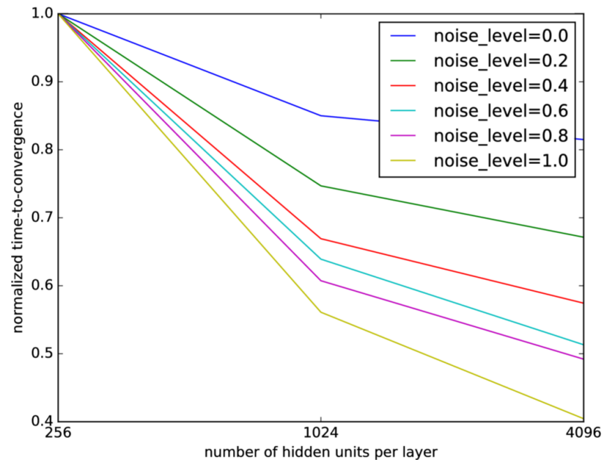
Time to convergence as a function of capacity with dataset size fixed to 50000
