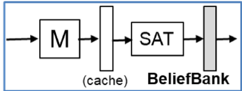
(B) constraint-solving
