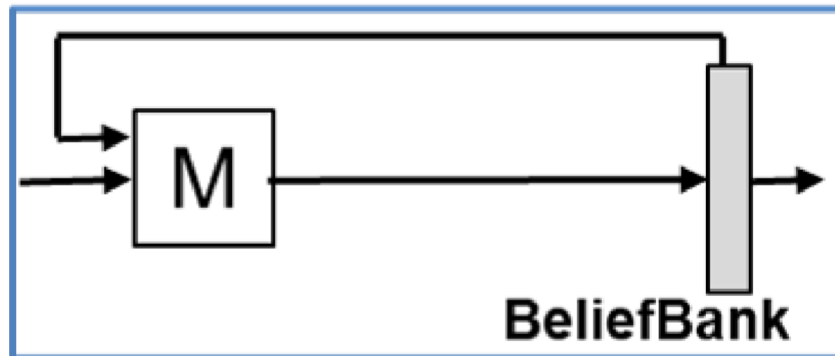
(C) feedback
