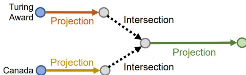
(B) Computation Graph
