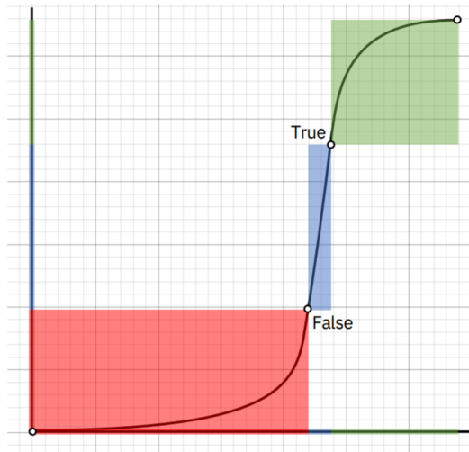
(b) A logistic activation function
