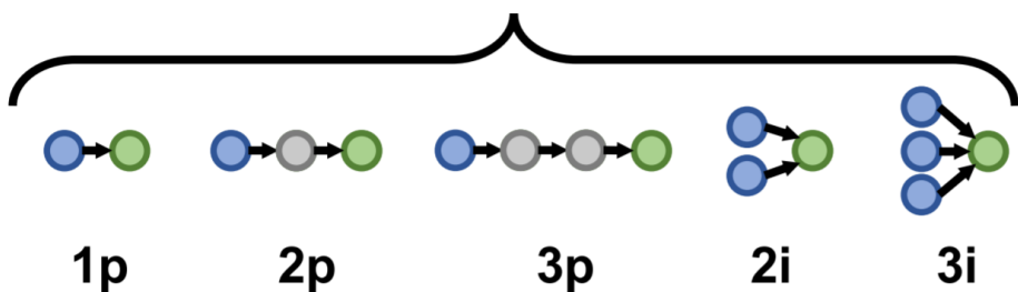
Training Conjunctive Queries
