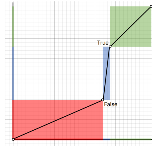
(c) A linearly interpolated activation function
