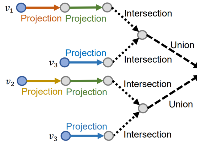
(B) Converted Computation Graph
