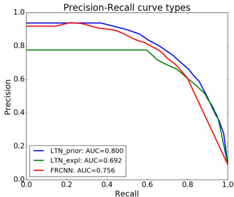
(a) LTNs with prior knowledge improve the performance of Fast R-CNN on object type classification, achieving an Area Under the Curve (AUC) of 0.800 in comparison with 0.756.
