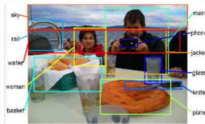
Ground Truth
