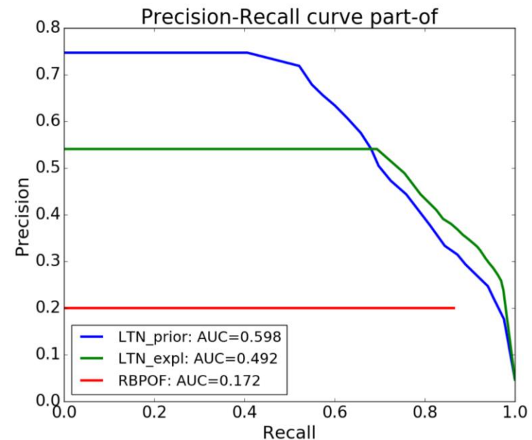
(b) LTNs with prior knowledge outperform the rule-based approach of Eq.2 in the detection of part-of relations, achieving AUC of 0.598 in comparison with 0.172.
