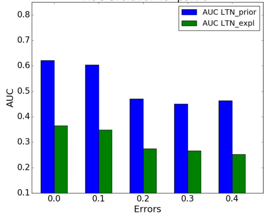
(b) Part-of predicate
