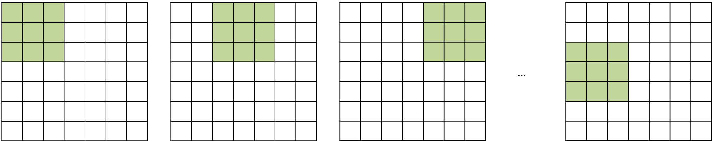
7x7 image / 3x3 filter / stride 2
