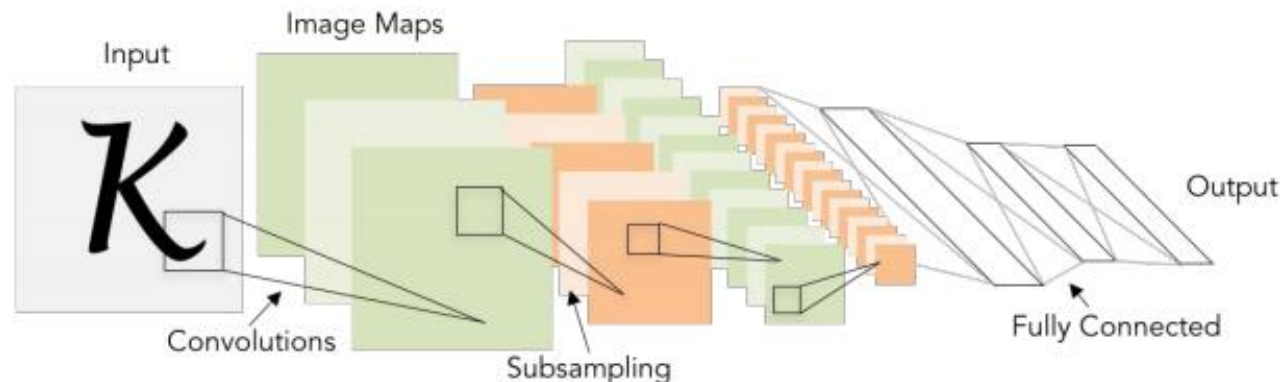
LeNet-5
