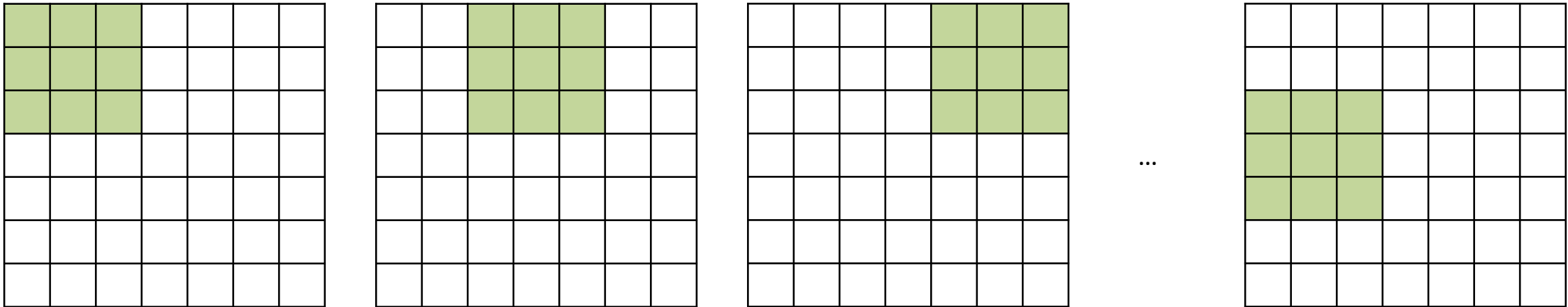
7x7 image / 3x3 filter / stride 2
