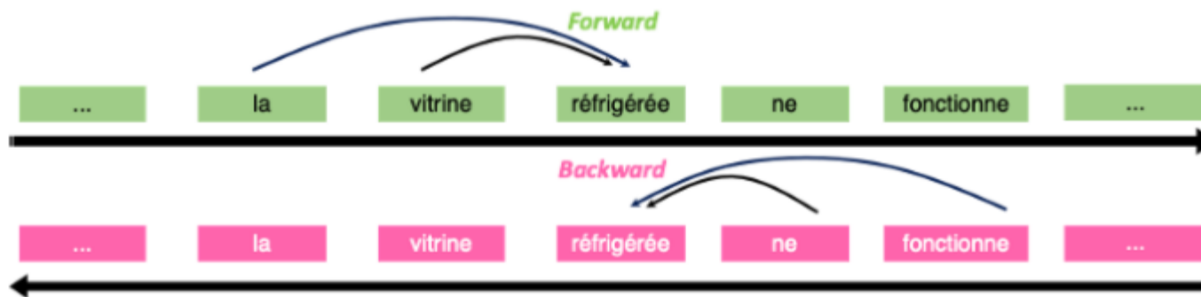
Autoregressive (AR) Language Model
