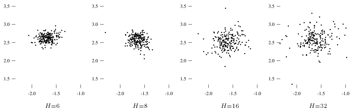
Figure 4.3: Predictive distributions obtained using networks of varying size. The plots show samples of 200 points from the predictive distributions based on training set A for the target values associated with inputs (2.0, 0.5), a point just outside the region of the training data, as defined by network models with 6, 8, 16, and 32 hidden units, using Gaussian priors. The 200 points were obtained using the networks from the last 200 super-transitions of the Markov chain Monte Carlo runs.
