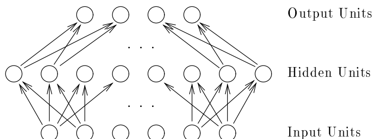
Figure 1.1: A multilayer perceptron with one layer of hidden units. The input units at the bottom are fixed to their values for a particular case. The values of the hidden units are then computed, followed by the values of the output units. The value of a unit is a function of the the weighted sum of values received from other units connected to it via arrows.
