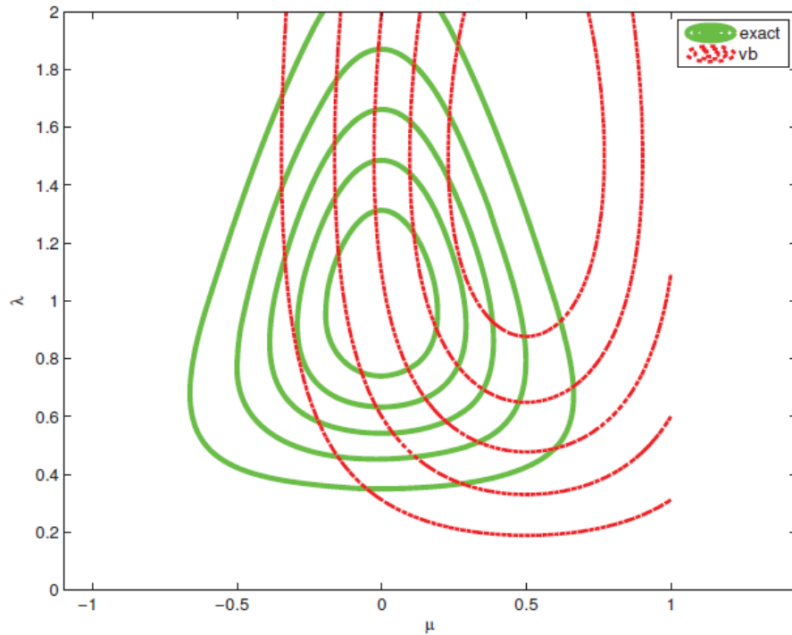
Initial guess
