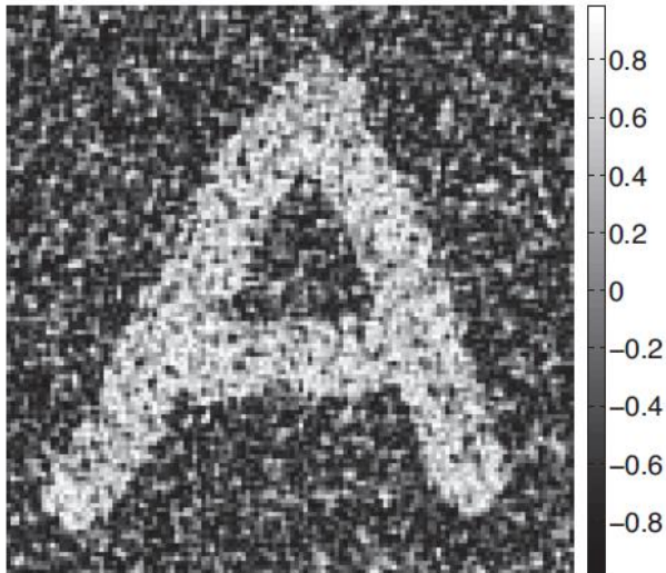
sample 1, meanfieldH
