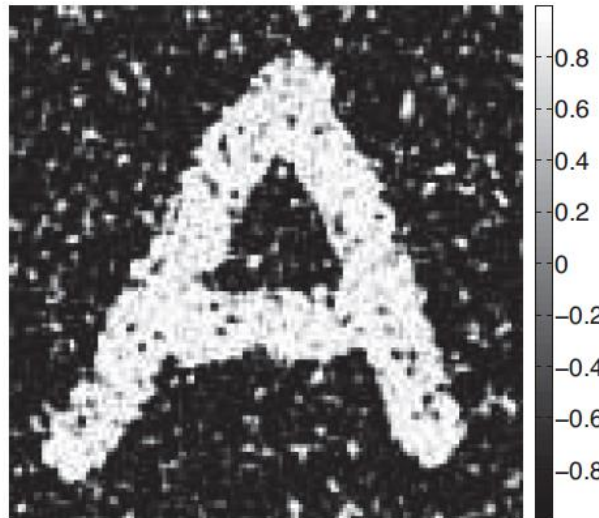
sample 3, meanfieldH
