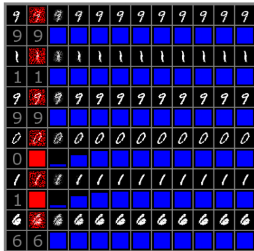
Figure 3: Mean field inference applied to MNIST digits. Within each pair of rows, the upper row shows pixels and the lower row shows class labels. The first column shows a complete, labeled example. The second column shows information to be masked out, using red pixels to indicate information that is removed. The subsequent columns show steps of mean field. The images show the pixels being filled back in by the mean field inference, and the blue bars show the probability of the correct class under the mean field posterior.
