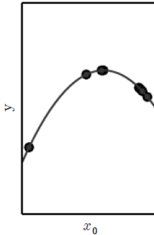
Appropriate capacity
