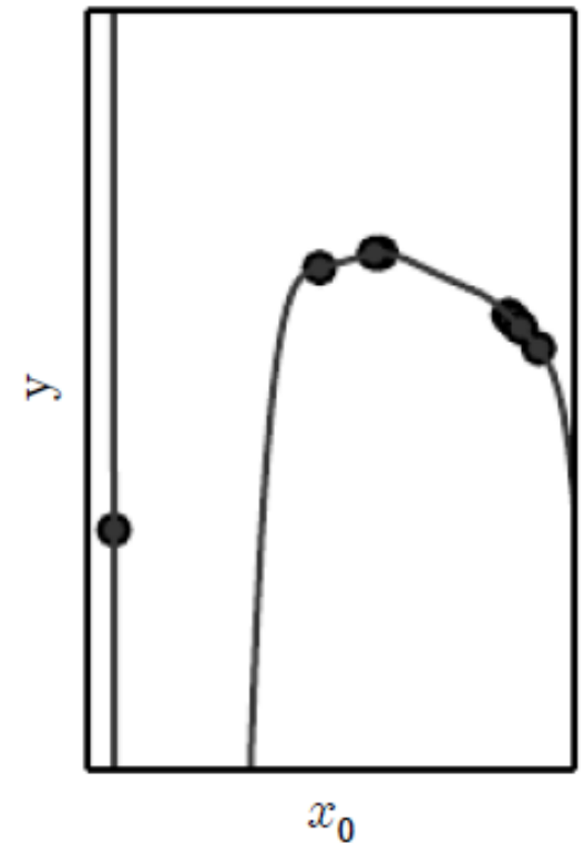
Overfitting
