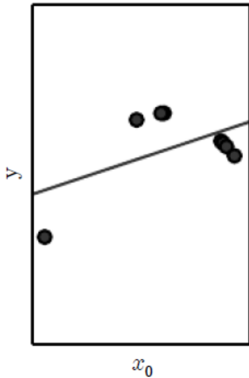
Underfitting
