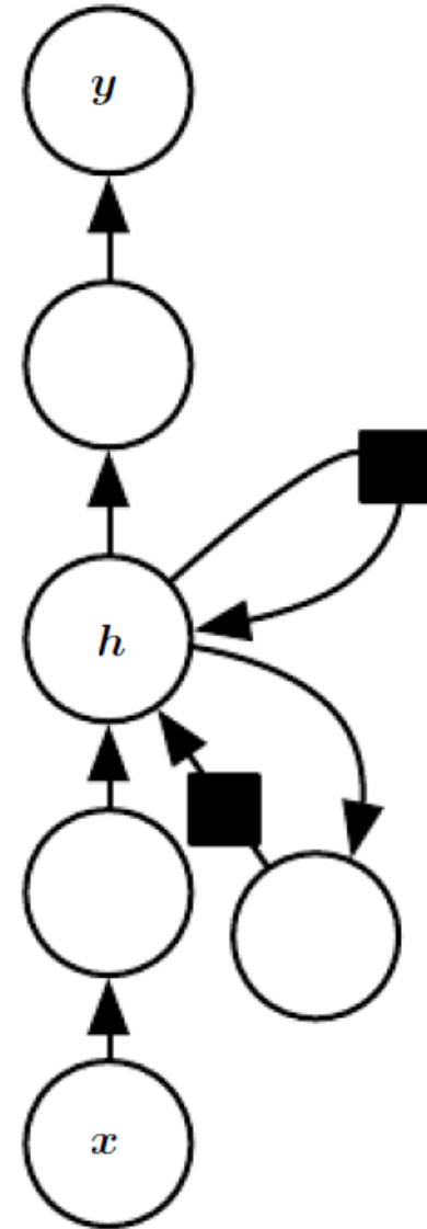
Skip connection
