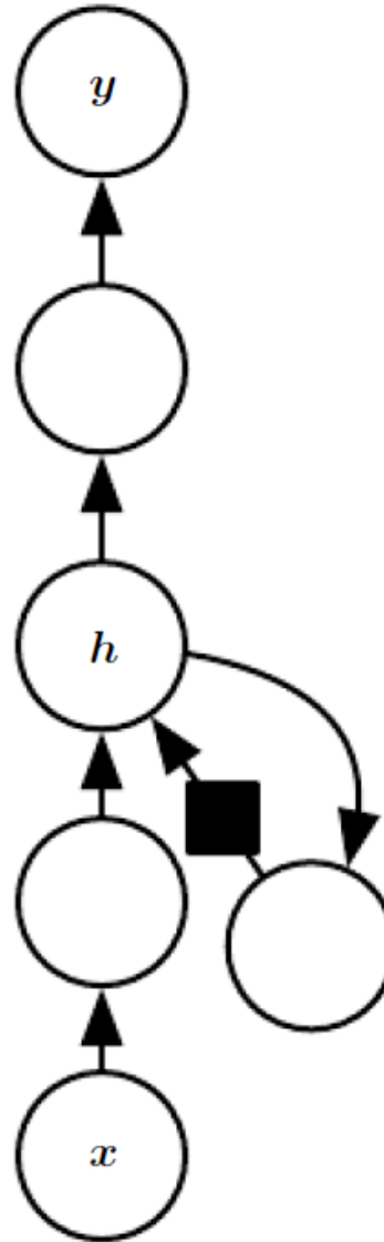
Deep computation
