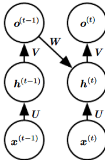
Test time
