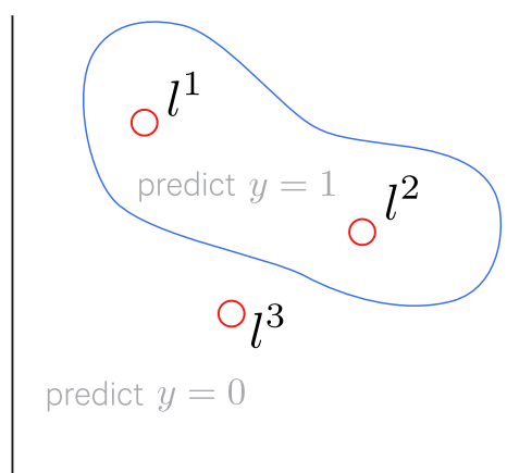
An example SVM decision boundary
