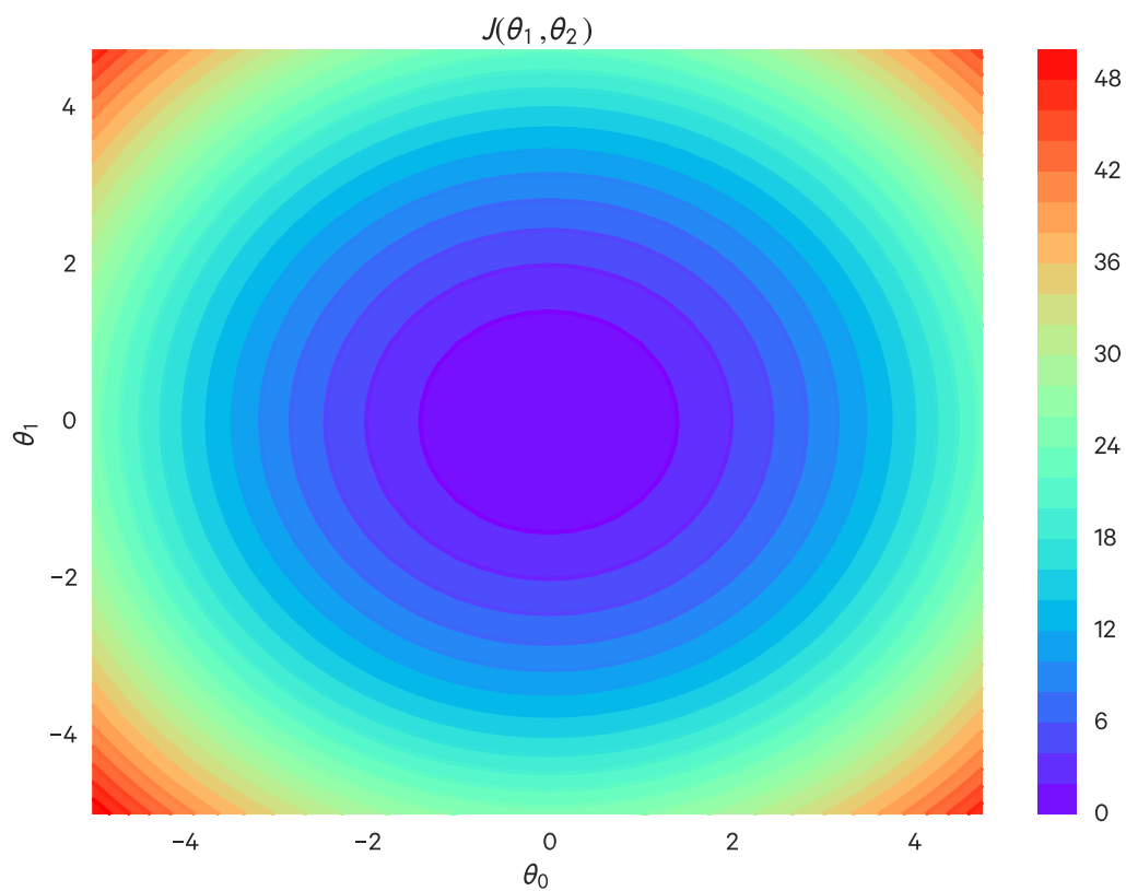
The same cost function, visualized as a contour plot
