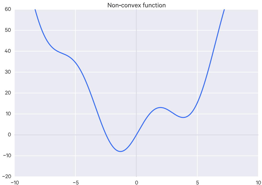
A non-convex function
