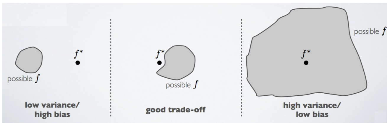
Bias and Variance
