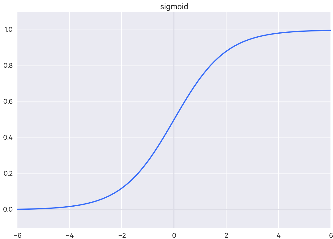
The sigmoid or logistic function
