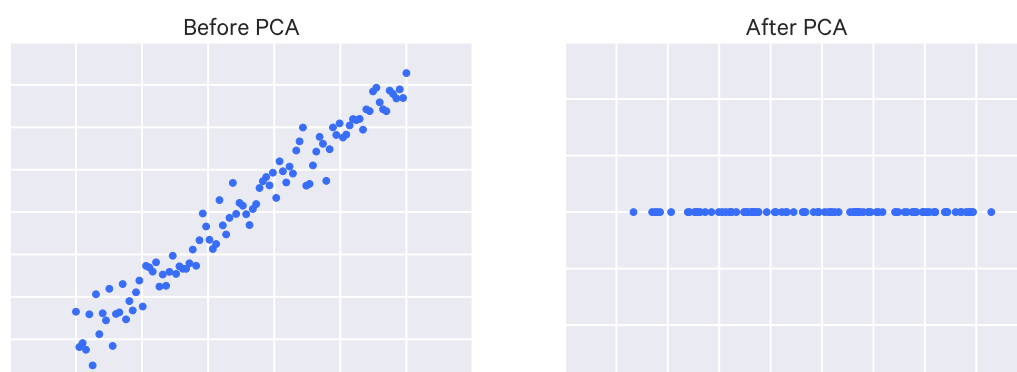
Reducing data dimensionality with PCA
