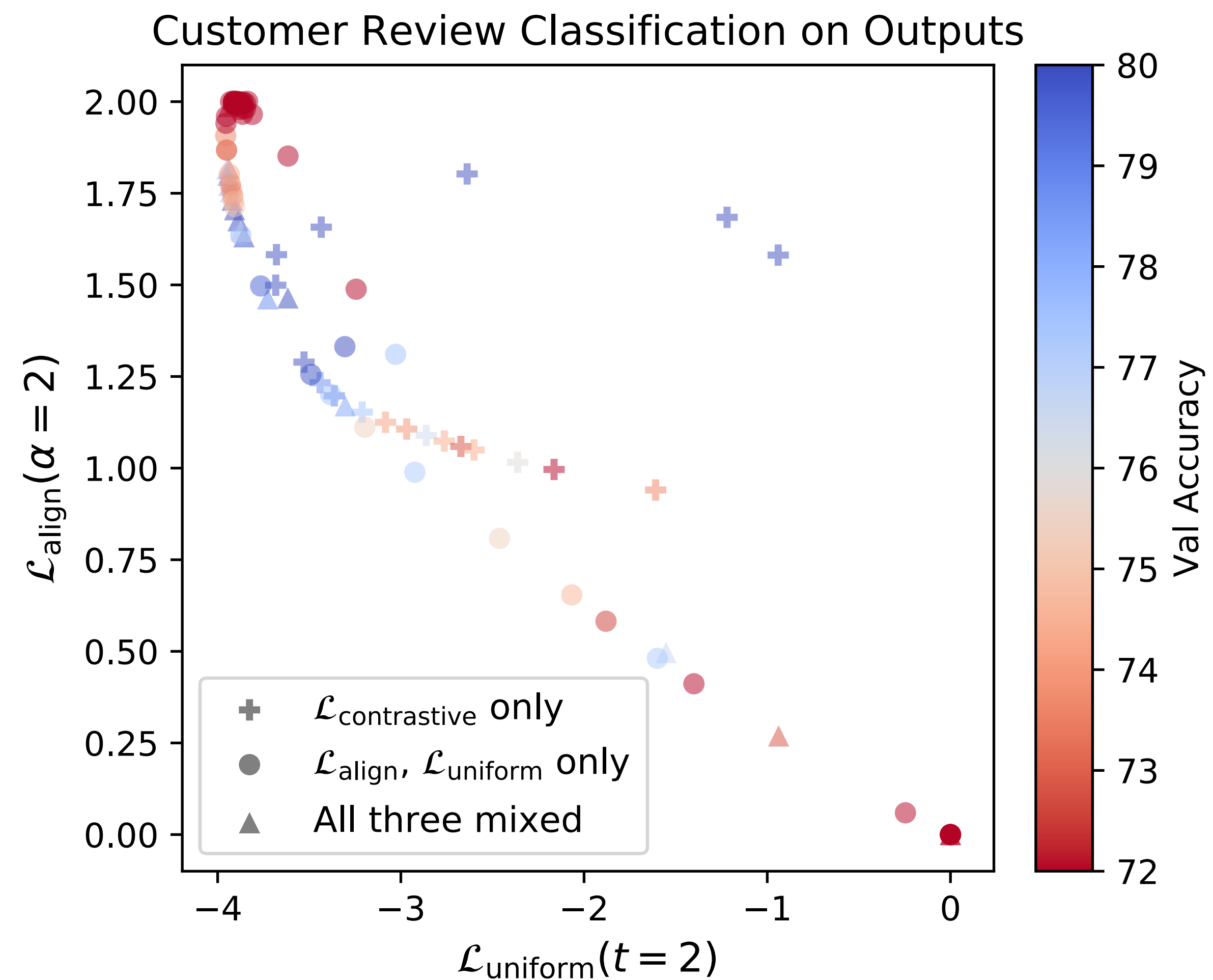
108 BookCorpus Encoders
