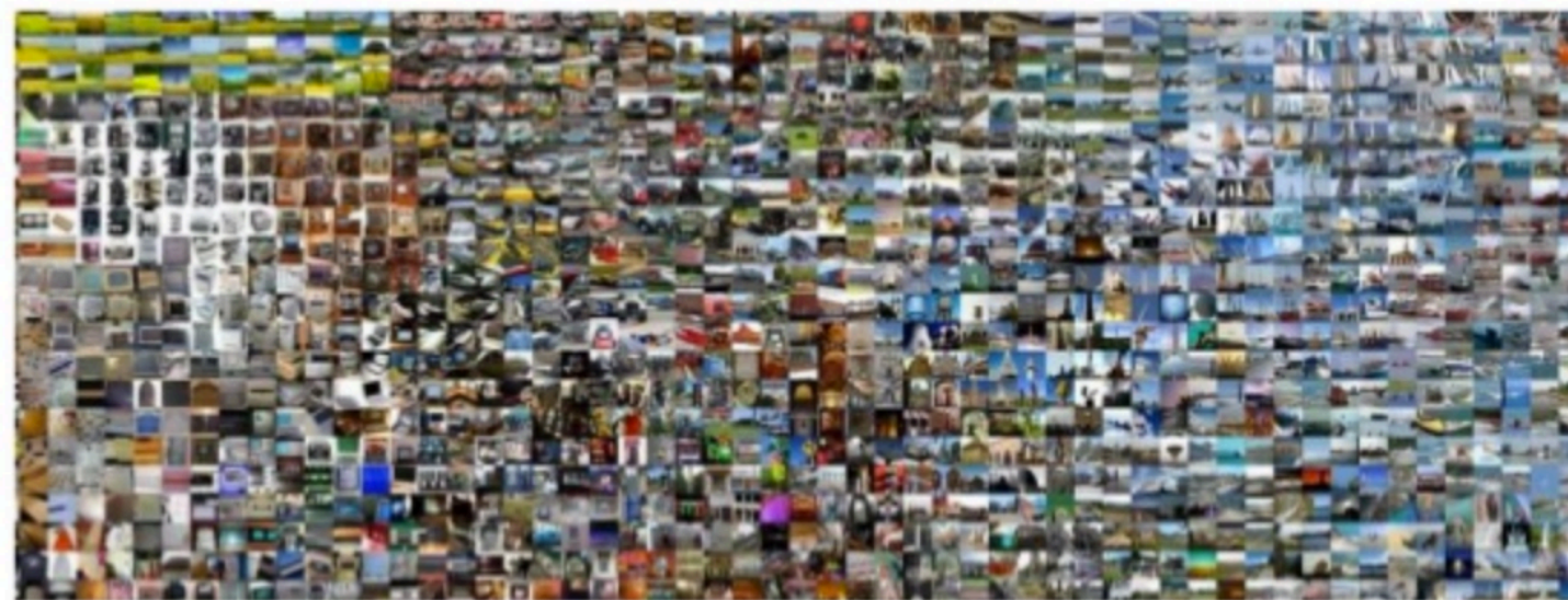
Image Classification
