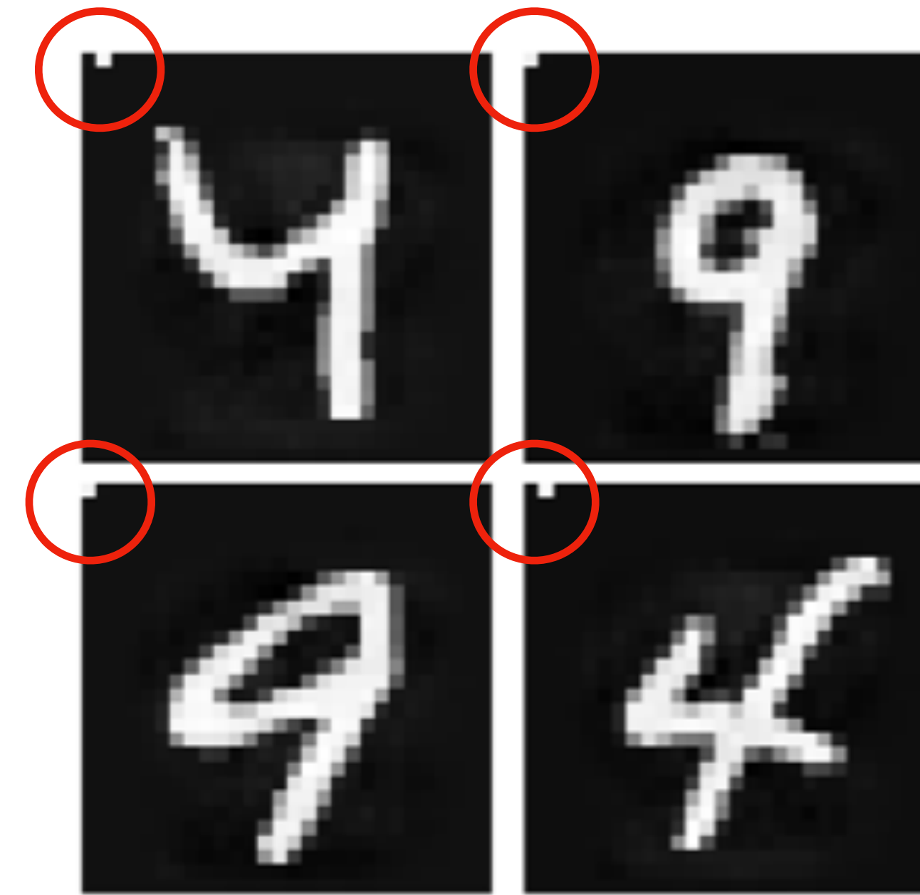
Adversarial perturbations
