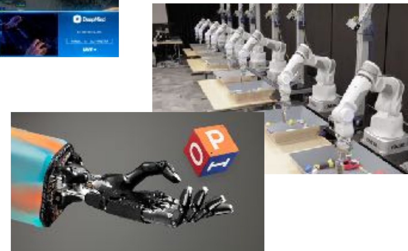
Robotic Manipulation
