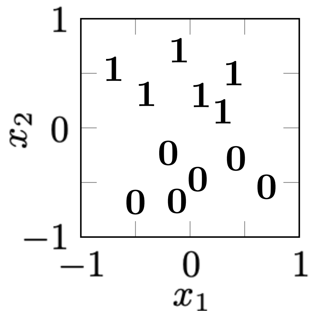
Training data
