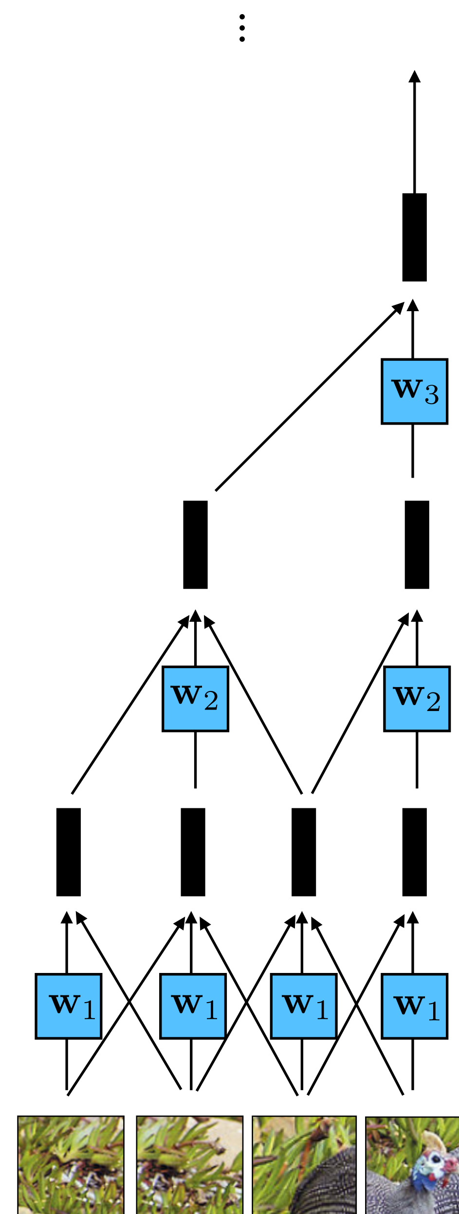
conv pyramid
