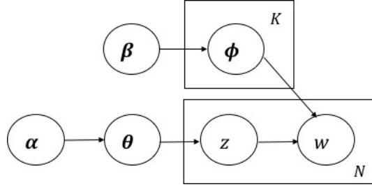
Figure 1: A graphical model for LDA
