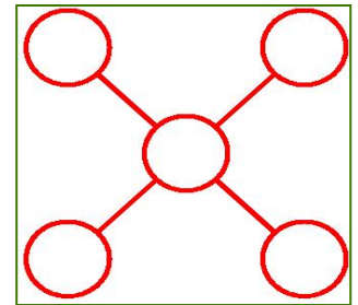
Undirected tree
