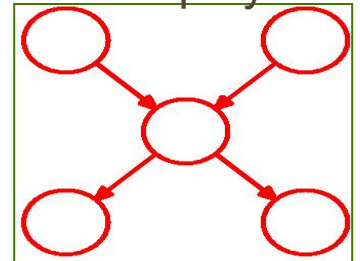
Directed polytree
