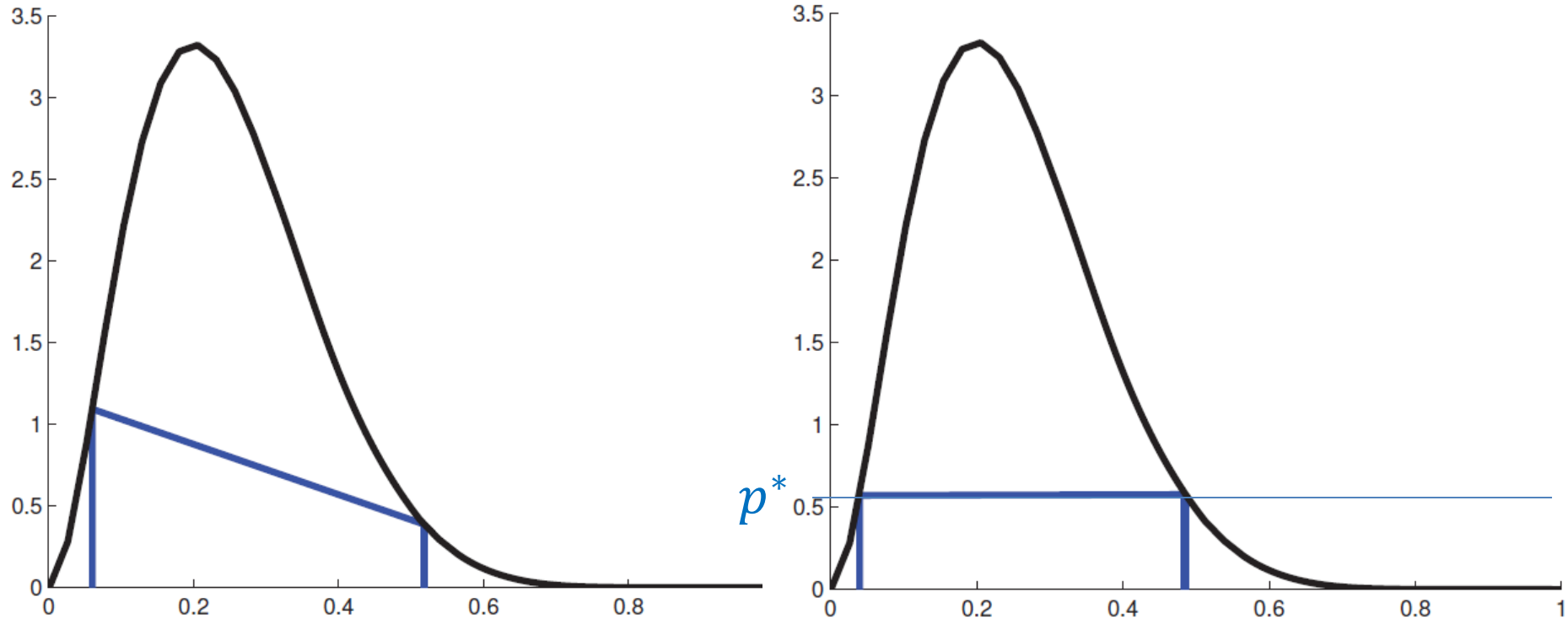
(a) Central interval and (b) HPD region for a Beta(3,9) posterior.
