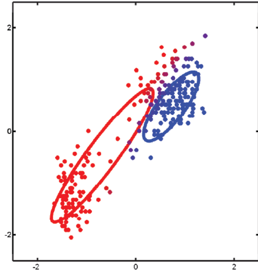
Iteration 5
