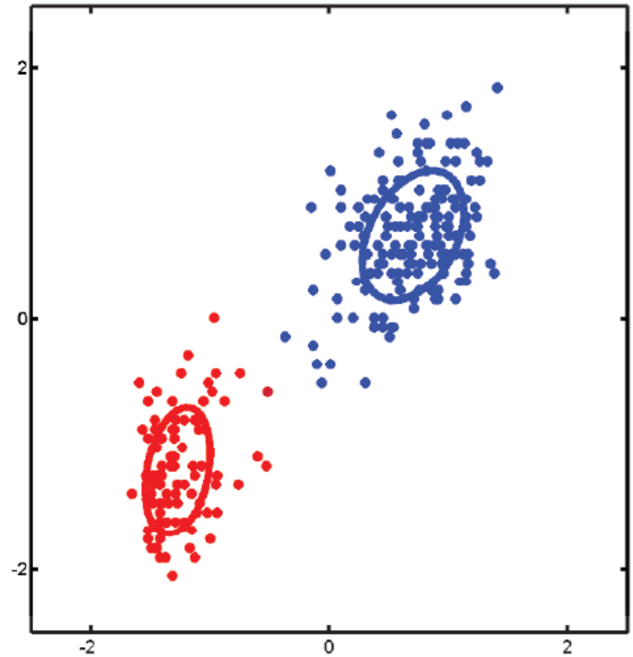
Iteration 16
