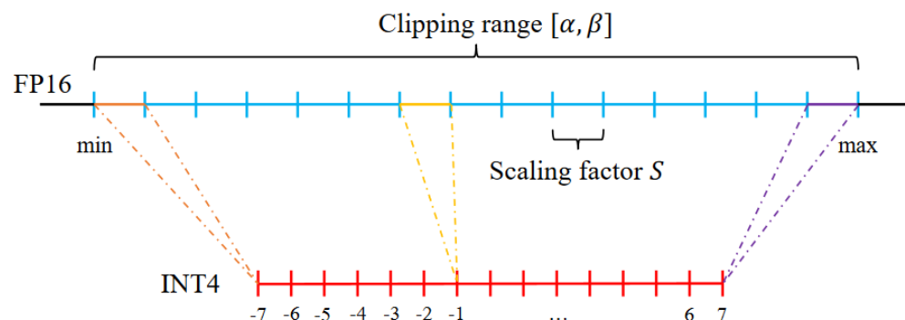
(a) Illustration of uniform quantization process
