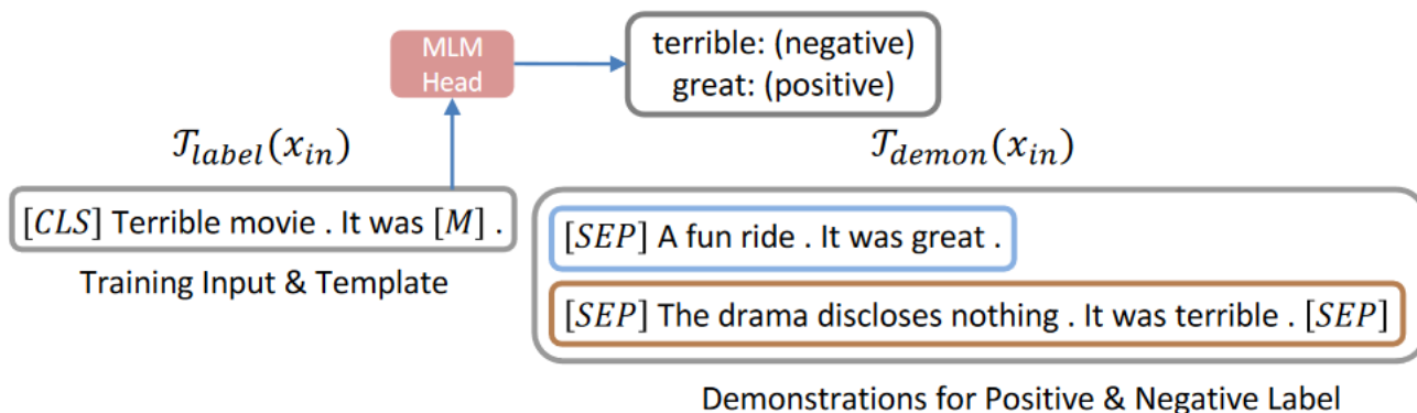
(a) Prompt-based fine-tuning with demonstration (LM-BFF)
